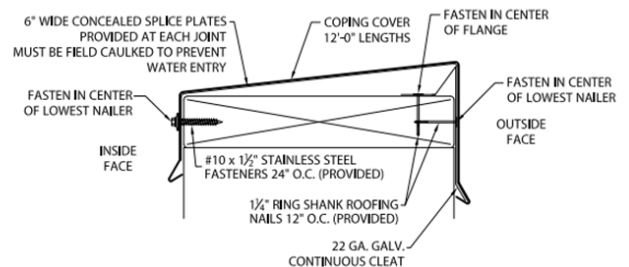
Typical Installation (Tapered Version)
