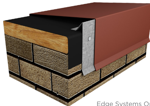
Edge Systems One One Coping (Flat Version)
