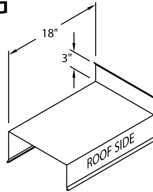
ENDWALL FLASHING COPING VERSION (RIGHT HAND SHOWN)
