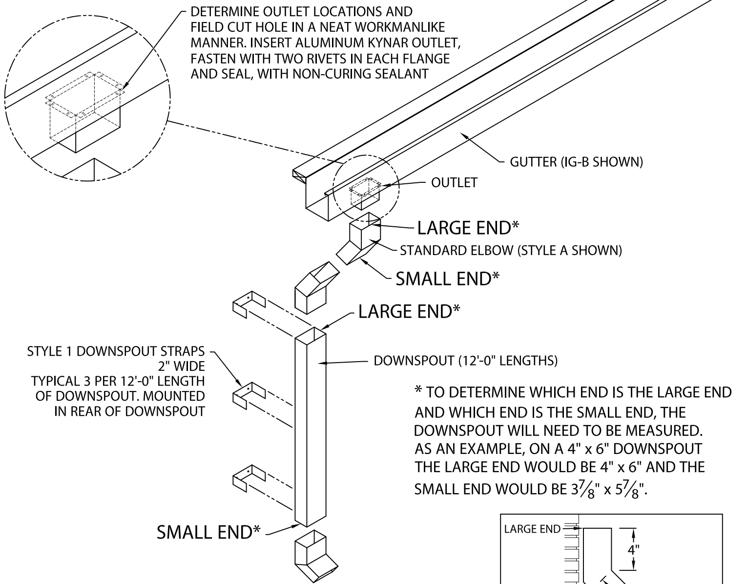
STYLE A DOWNSPOUT
