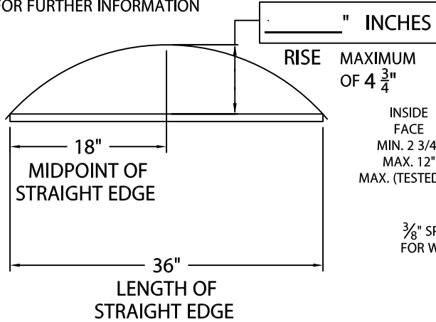
DETAIL A
