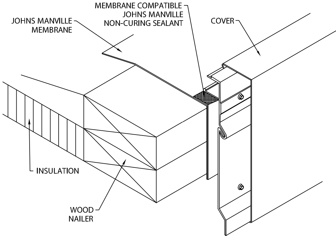
TYPICAL OVERVIEW
