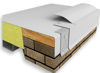
← TPO or PVC Skirted (Factory Applied TPO or PVC Flashing)
