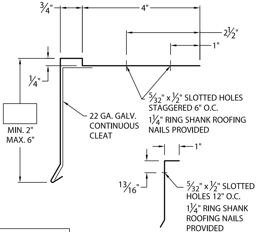
CLEAT DETAIL
