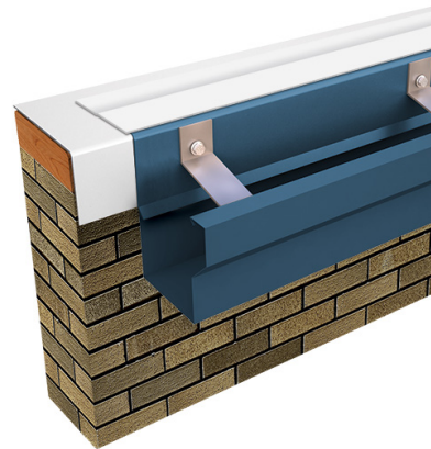
Seal-Tite Industrial Gutter (IG-1)
