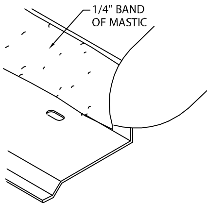
BASE RAIL SHOWN WITH INSIDE FACE UP.
