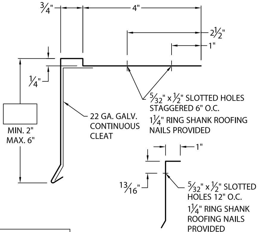
CLEAT DETAIL
