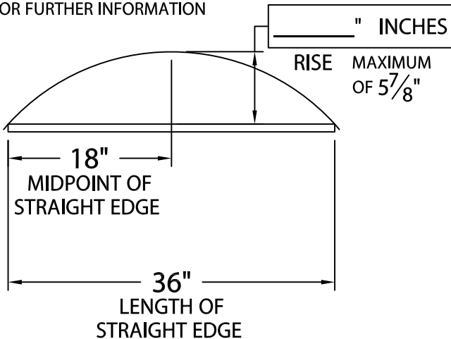
DETAIL A
