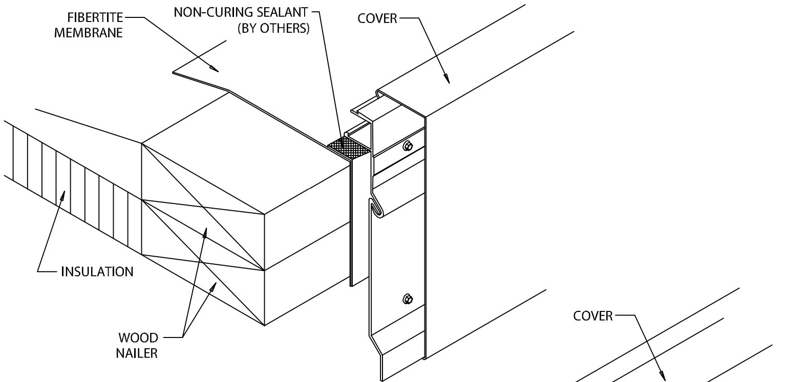
TYPICAL OVERVIEW
