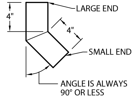
STANDARD ELBOW
