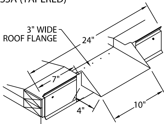
SPILLOUT SCUPPER TYPE SSA (TAPERED)
