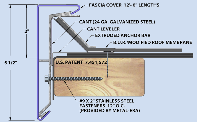
FiberTite AT Canted Fascia Existing Cant & Galvanized Waterdam (shown) Versions .050" & .063" fascia cover
