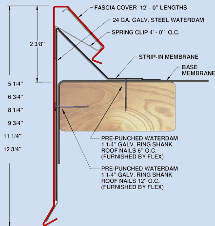
FiberTite 200 Fascia Fully Adhered or Mechanically Attached Single-Ply (Shown) & Stone Ballast Versions 24 ga., .040", .050", .063" fascia cover
