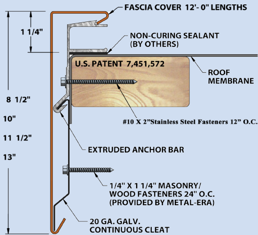
FiberTite AT Extended Fascia Fully Adhered or Mechanically Attached Single-Ply Version .050" & .063" fascia cover
