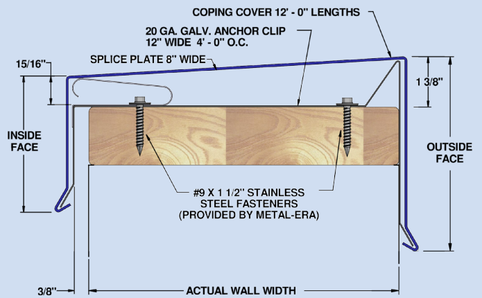
FiberTite Coping Tapered, Flat or Existing Versions 24ga., .040", .050", .063" coping cover
