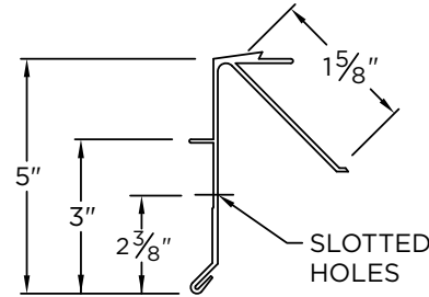
EXTRUDED PROFILE
