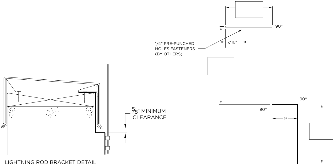
LIGHTNING ROD BRACKET DETAIL
