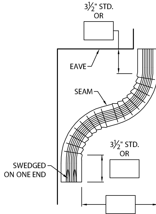
STYLE "A" OFFSET EAVE CONDITION
