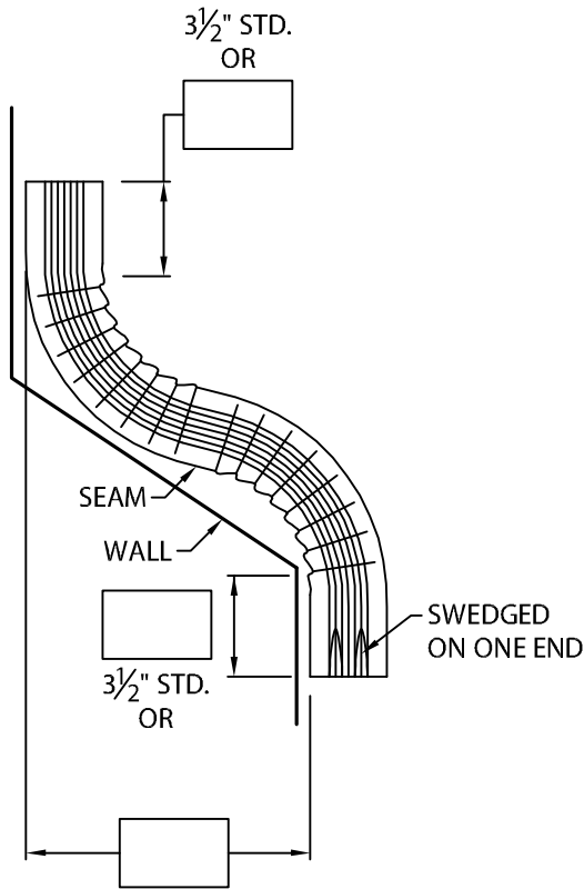
STYLE "A" OFFSET WALL CONDITION
