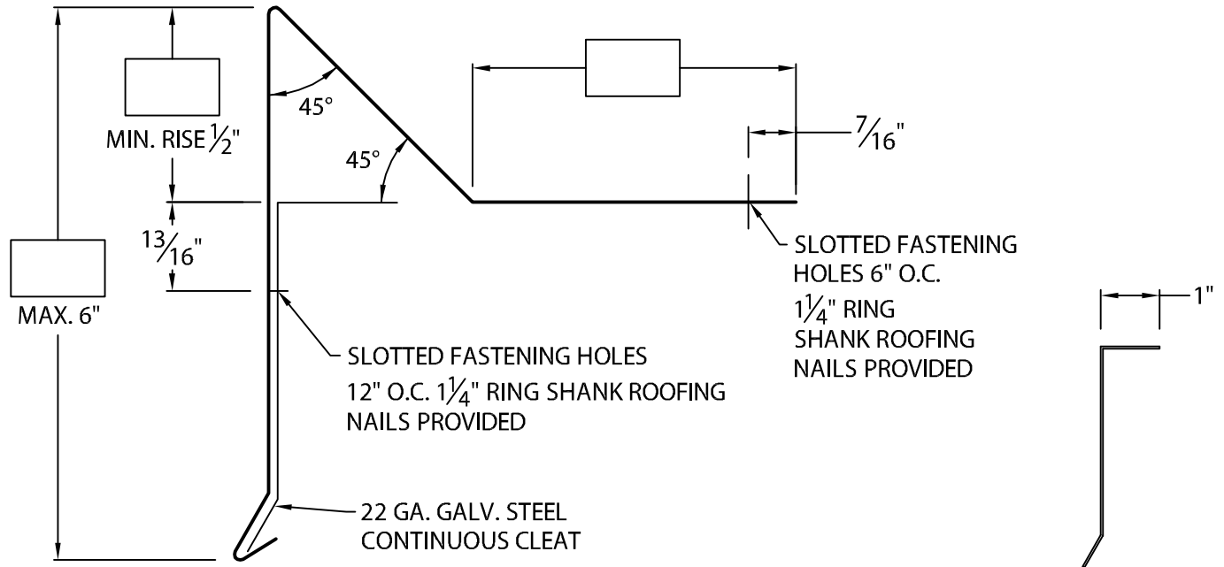
CLEAT DETAIL
