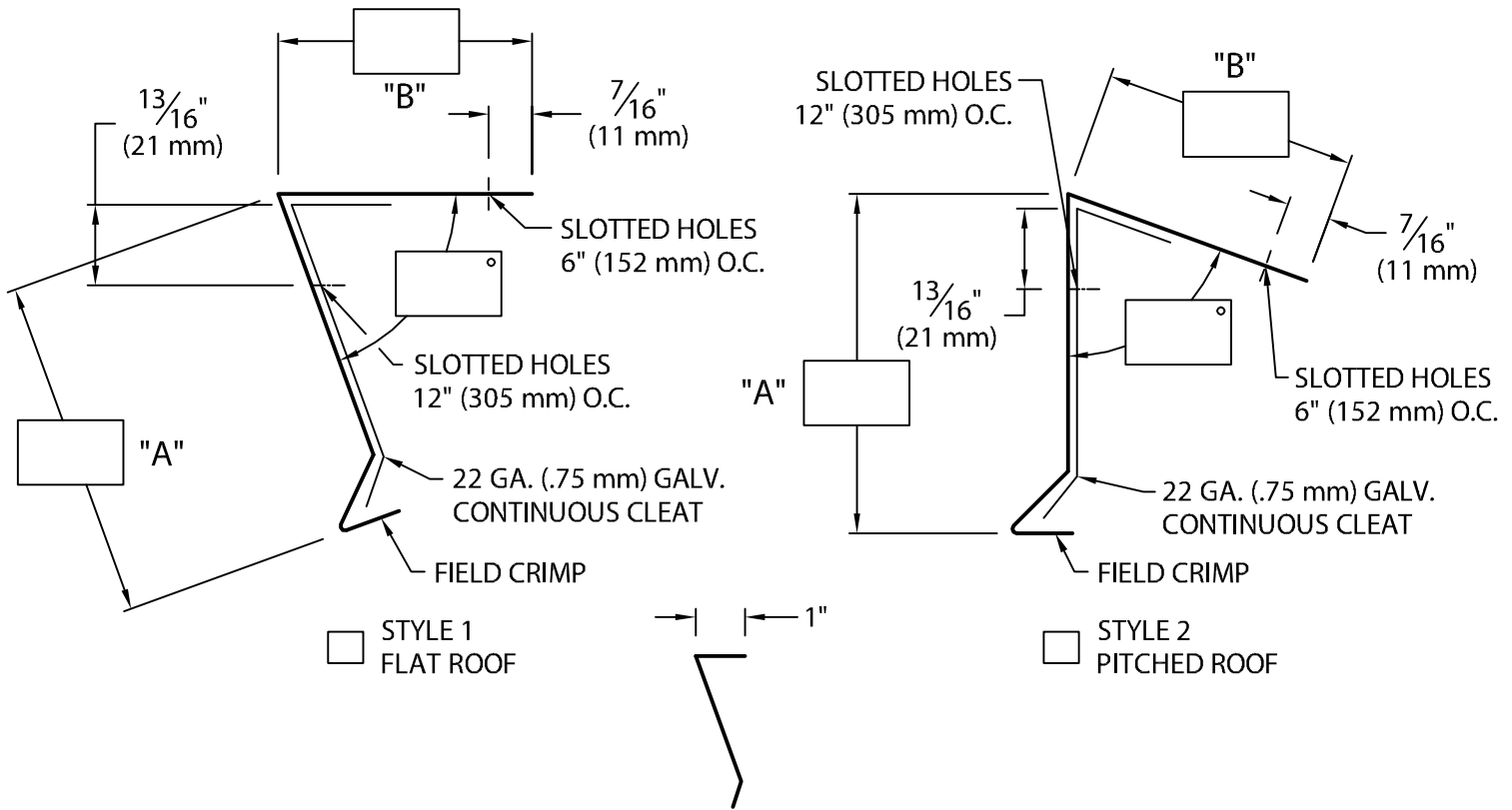
CLEAT DETAIL (TYP.)
