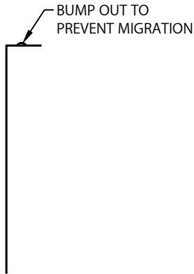
COVER SPLICE PLATE 3½" WIDE
