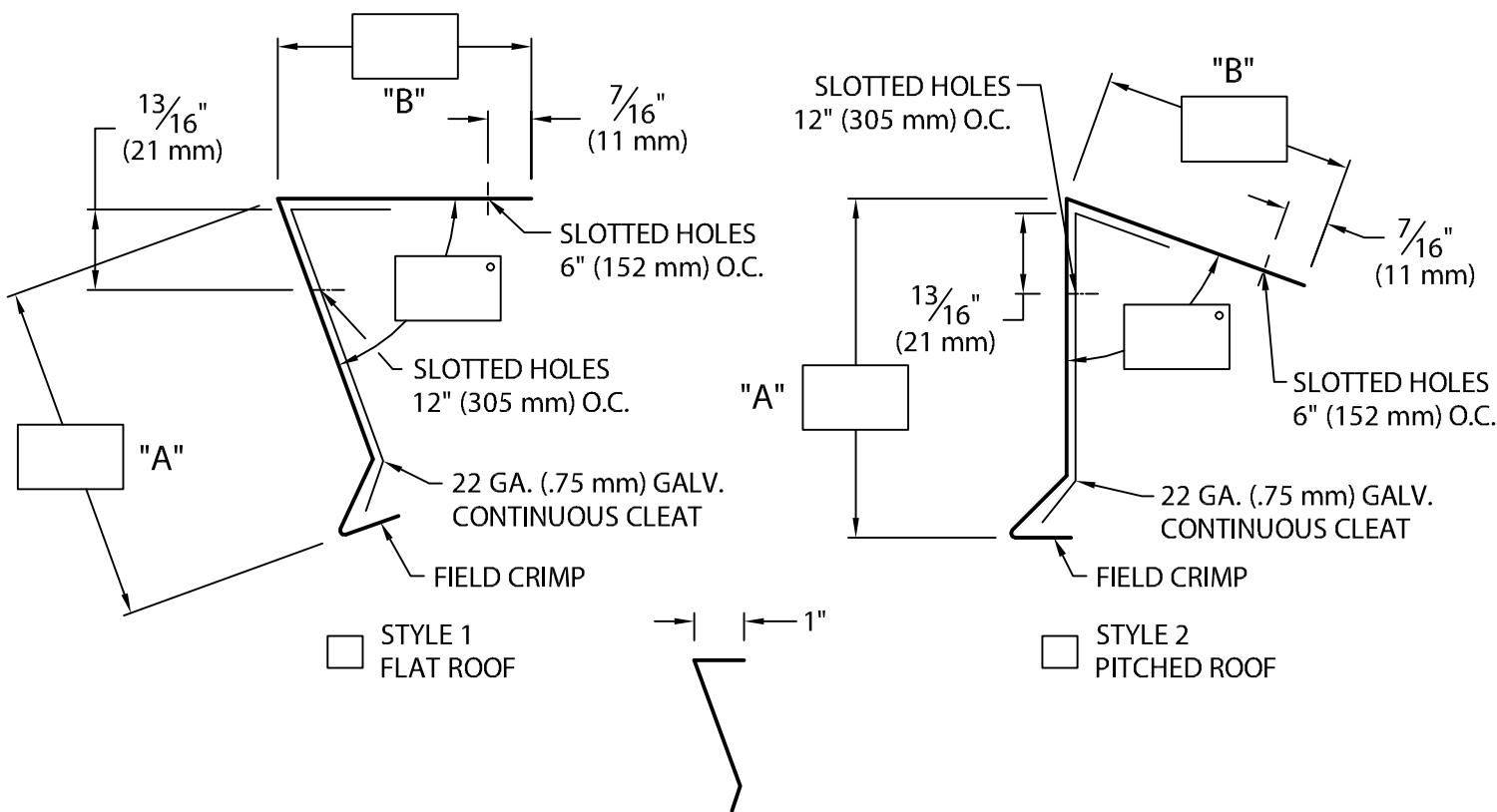
CLEAT DETAIL (TYP.)
