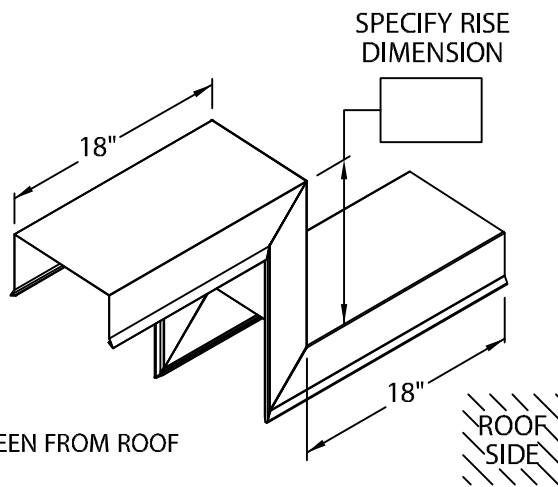
RIGHT HAND STEP-UP MITER
