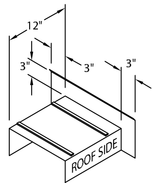
ENDWALL FLASHING SPLICE PLATE VERSION (RIGHT HAND SHOWN) (AVAILABLE ONLY IN .040\"/>
