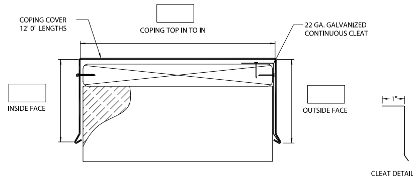
ONE COPING FLAT VERSION
