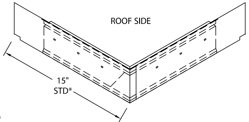
2-PC. SNAP-ON COVER
