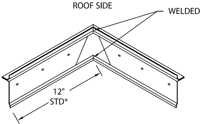
1-PC. RETAINER GUARD
