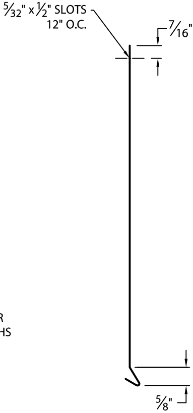
COVER DETAIL
